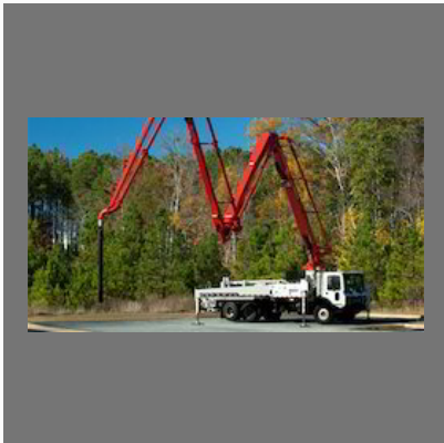
Boom Pump Pipes 4.5mm to 7.5mm Thickness Available
