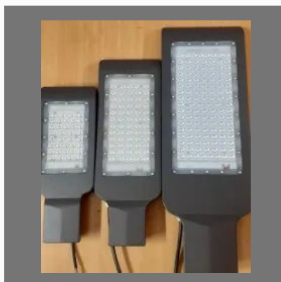
LED Street Light withlen's 100w
