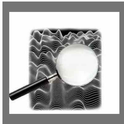
Image Processing
