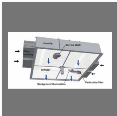
Laminar Air Flow
