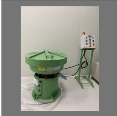
Vibratory Finishing Machine (150 liters)
