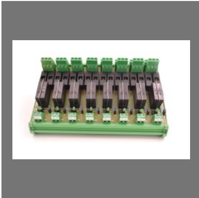
Double Changeover Relay Module - 8 Channel Module
