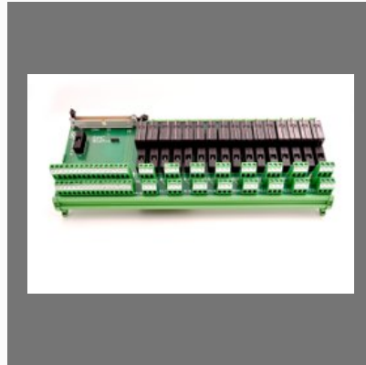
Input - Output Relay Module - 16 Channel Module
