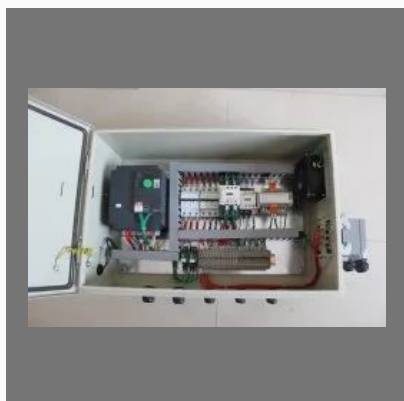
EOT CRANE CONTROL PANEL
