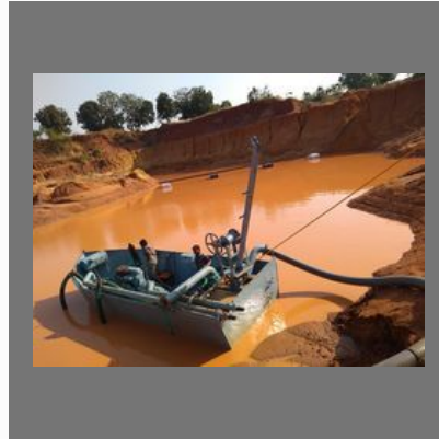
Sand Dredging Pump Set
