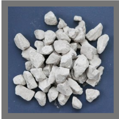
Calcium Oxide
