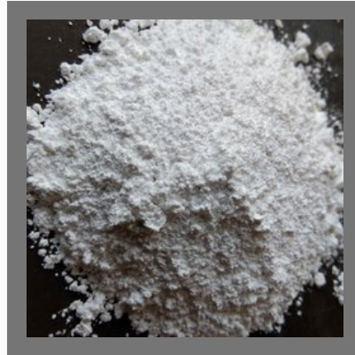
Calcium Hydroxide
