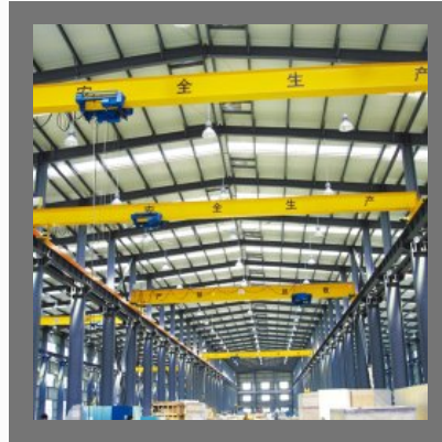
Hot Cranes
