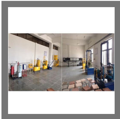
Fluid Machinery Lab
