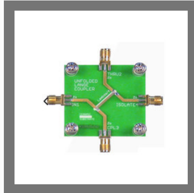
4G Ready 0.04-4 GHz RF & MIC Training Lab MIC04
