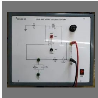
Wein Bridge Oscillator Trainer kit
