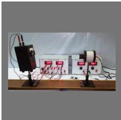
Photo- Electric Effect Apparatus
