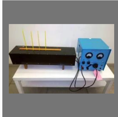
Angstrom Method of Thermal Conductivity
