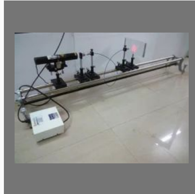
Numerical Aperture of A Fiber
