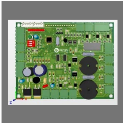
MAG-DEMAG Controller
