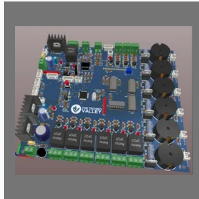
Three Phase Thyristor (SCR) Controller Card
