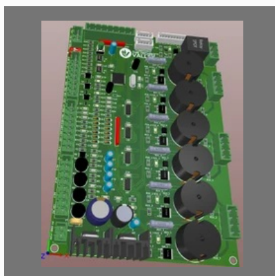
Electrocoagulation SCR Controller Board
