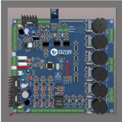
Water Treatment Controller Board
