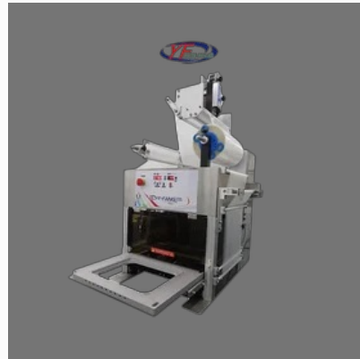
Y fang - Table Type MAP Sealing Machine-ET-900LF
