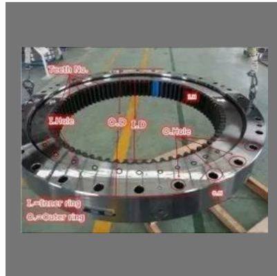
Excavator Swing Bearing
