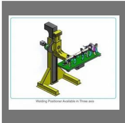
Welding Positioner Available in Three axis
