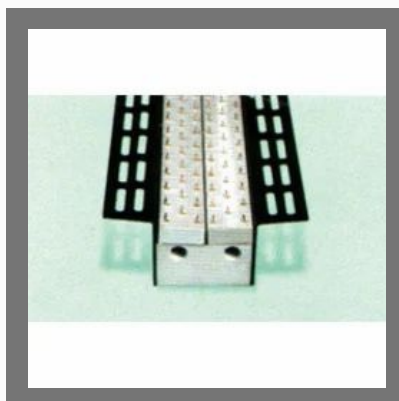
RSK Beater Pinned Beater Segment & Wired Beater Segment
