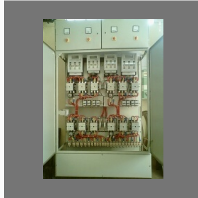
Motor Control Center
