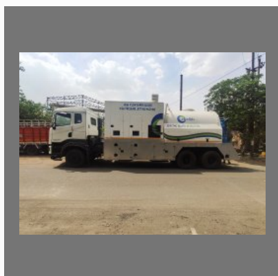
Swachhta Super Sucker Machine with Dump Tank
