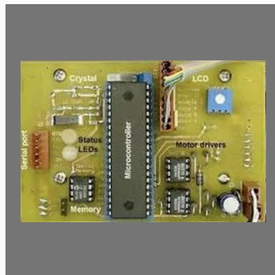
Microcontroller Training Kit
