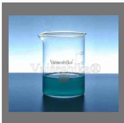
Glass Beaker
