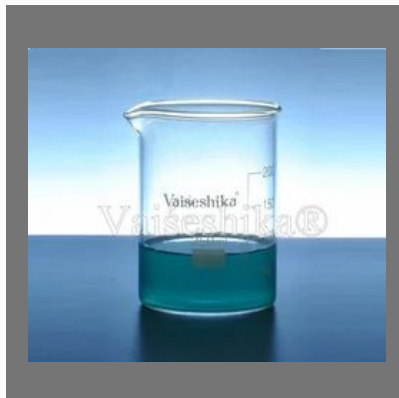
Glass Beaker
