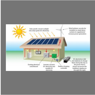
Rooftop Solar System
