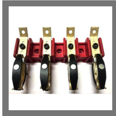
Female Male contact Assembly
