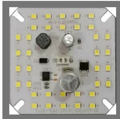
Mc Pcb Board
