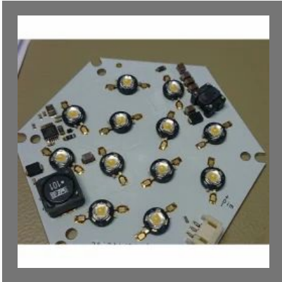
LED Metal Clad PCB
