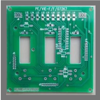
Single Layer PCB
