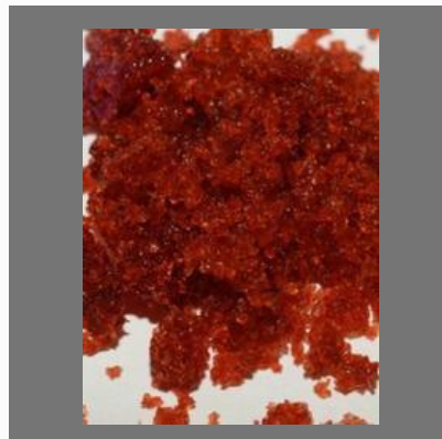
COBALT NITRATE
