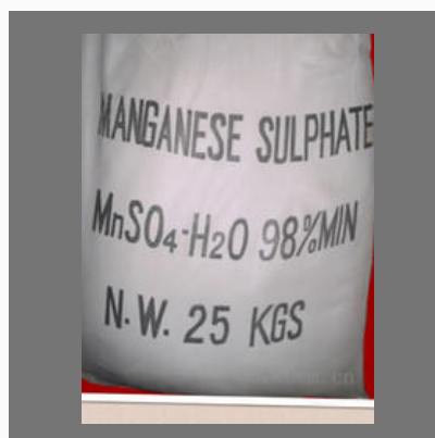
Manganese Sulphate
