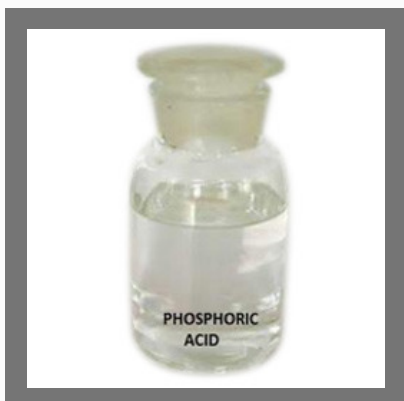
Phosphoric Acid
