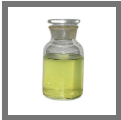
Sodium Hypochlorite
