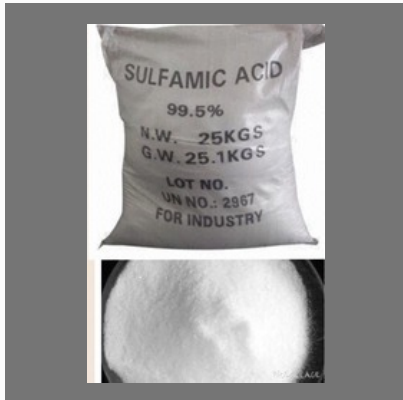
Sulfamic Acid
