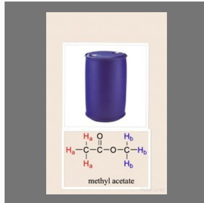
Methyl Acetate
