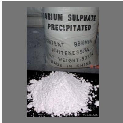
Barium Sulphate
