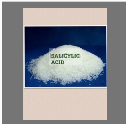
Salicylic Acid
