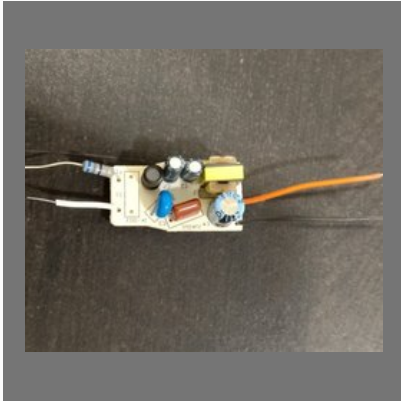
LED Bulb Driver 3-9w
