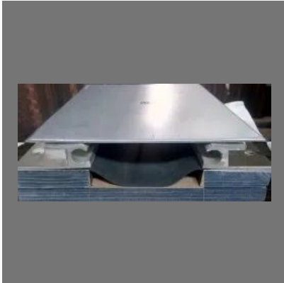
VRE Floor Expansion Joint System
