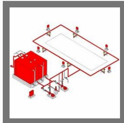
Pressurized Fire Hydrant System
