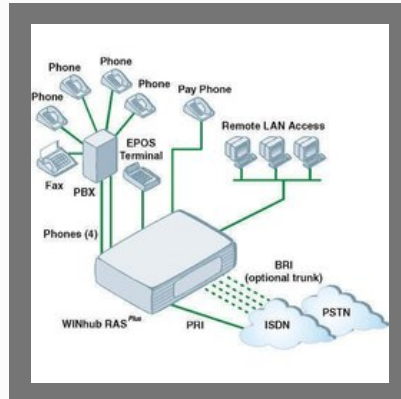
PRI Connection Provider
