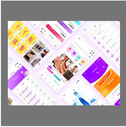
Ecommerce Application
