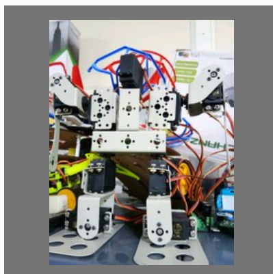
Robot
