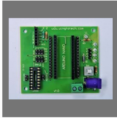
Robotics Development Board With Arduino Nano And L293d Ic Slot
