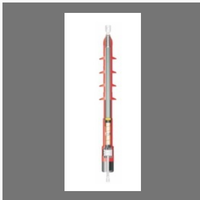
11 KV (UE) / 22 KV(E) Heat Shrinkable Terminations 1 Core
