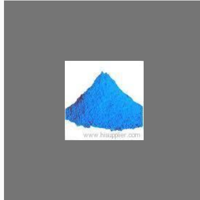
Vanadium Sulphate
