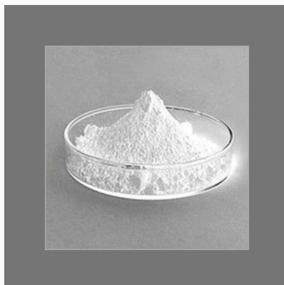
Mercuric Chloride
