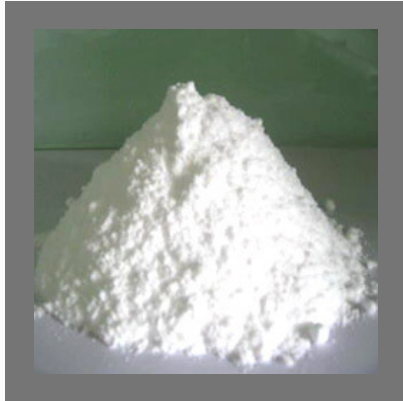
Ammonium Molybdate
