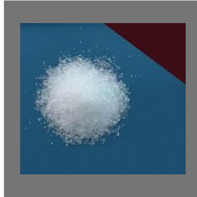
Ca-Calcium Nitrate
