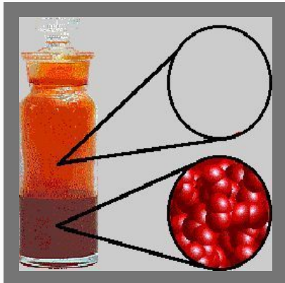
Liquid Bromine
