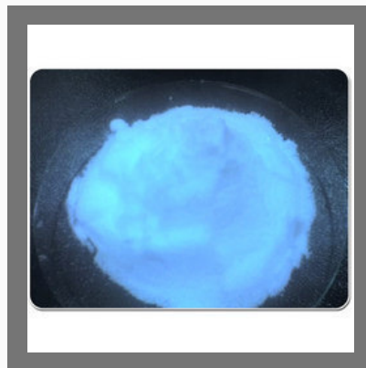
Mercuric Sulphate
