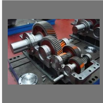
Gearbox Repair
